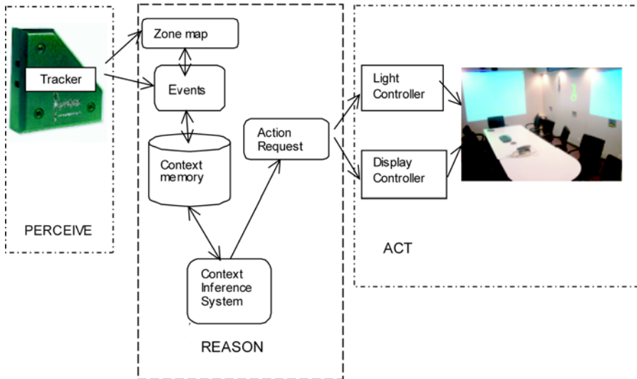
Fig. 11. System architecture
